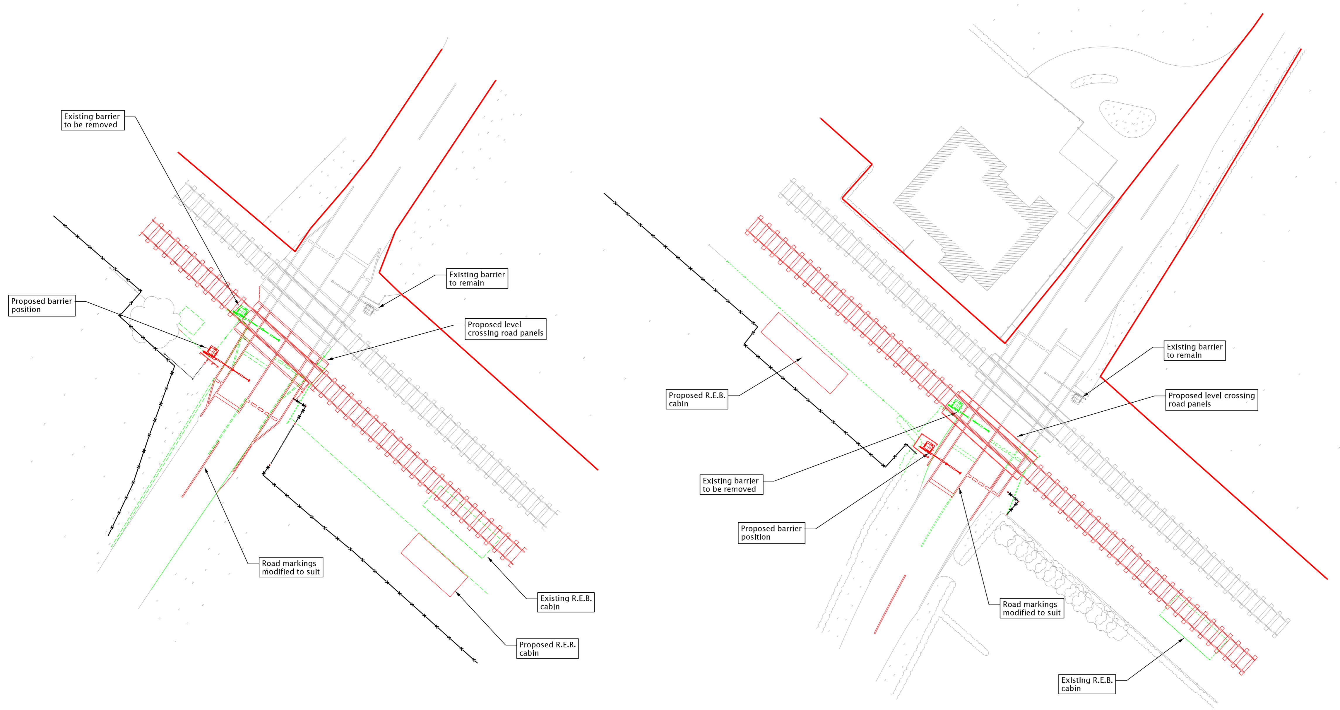
PLAN ON LEVINGTON LEVEL CROSSING
